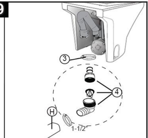
Horizontal Installation
